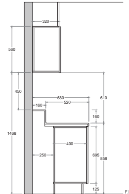
Cabinetry Section
