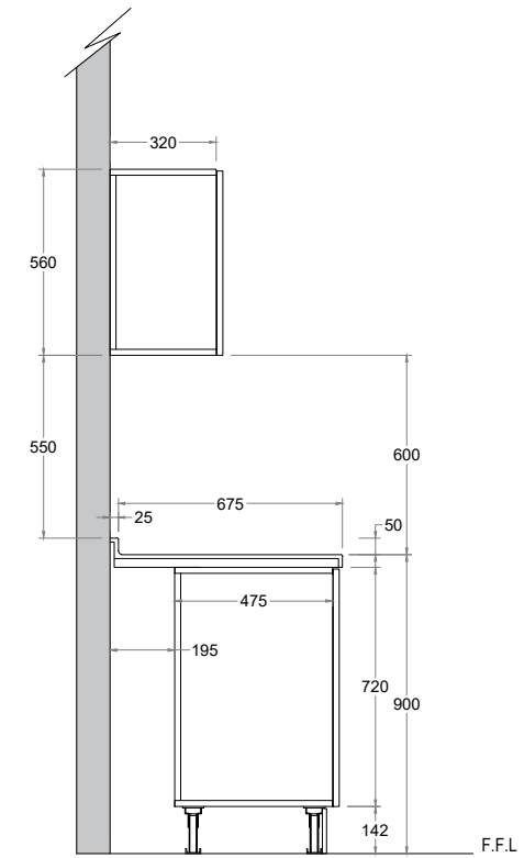
TYPICAL SECTION - LDU
